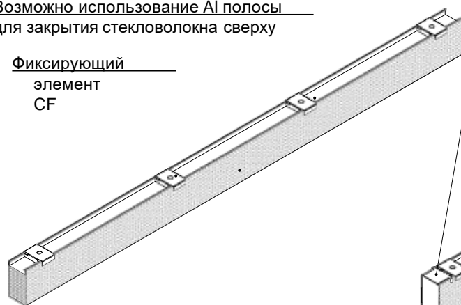
Рейка AR C WP
